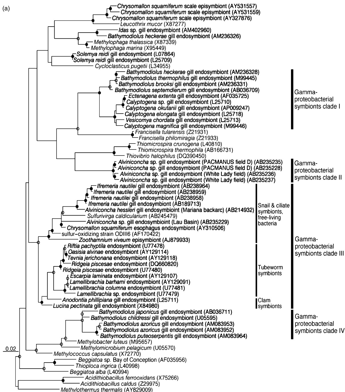
Fig. 1. 16S rRNA gene-based trees showing the major mesophilic deep-sea vent chemoautotrophs. The trees were constructed, evaluated and optimized using the ARB program (Ludwig et al. , 2004). Chemoautotrophic symbionts are indicated in bold type. GenBank/EMBL accession numbers are shown in parentheses. The scale bars represent the expected number of changes per nucleotide position. Distances were estimated with the Jukes–Cantor correction. Bootstrap analyses with 100 trial replications were used to obtain confidence estimates for the tree topologies. Branch points conserved with bootstrap values of > 75% (●) and with bootstrap values of > 50% (○) are indicated. (a) Tree showing the relationships among members of the Gammaproteobacteria. Unambiguously aligned positions (945 bases) were used. (b) Tree showing the relationships among members of the Epsilonproteobacteria. Unambiguously aligned positions (1026 bases) were used.
