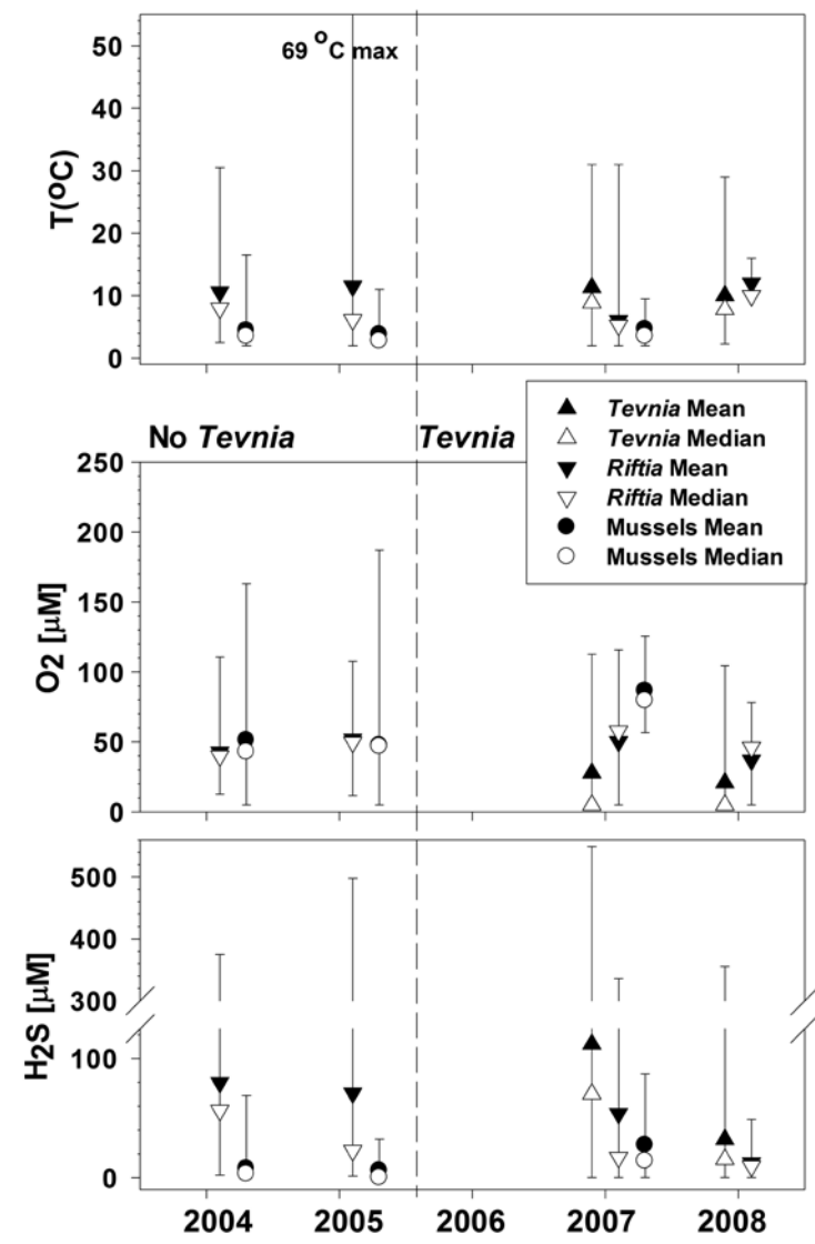
Figure 4. Mean, median, minimum, and maximum temperature, O 2 , and H 2 S data for 9°N on the East Pacific Rise (9 N EPR) from 2004–2008. The data represent over 3,000 electrochemical scans using DSV Alvin. Minimum and maximum data are the low and high points of the solid vertical lines. The dashed vertical line represents the start of the eruptions. The year corresponds to year of data collection and not the true date.
