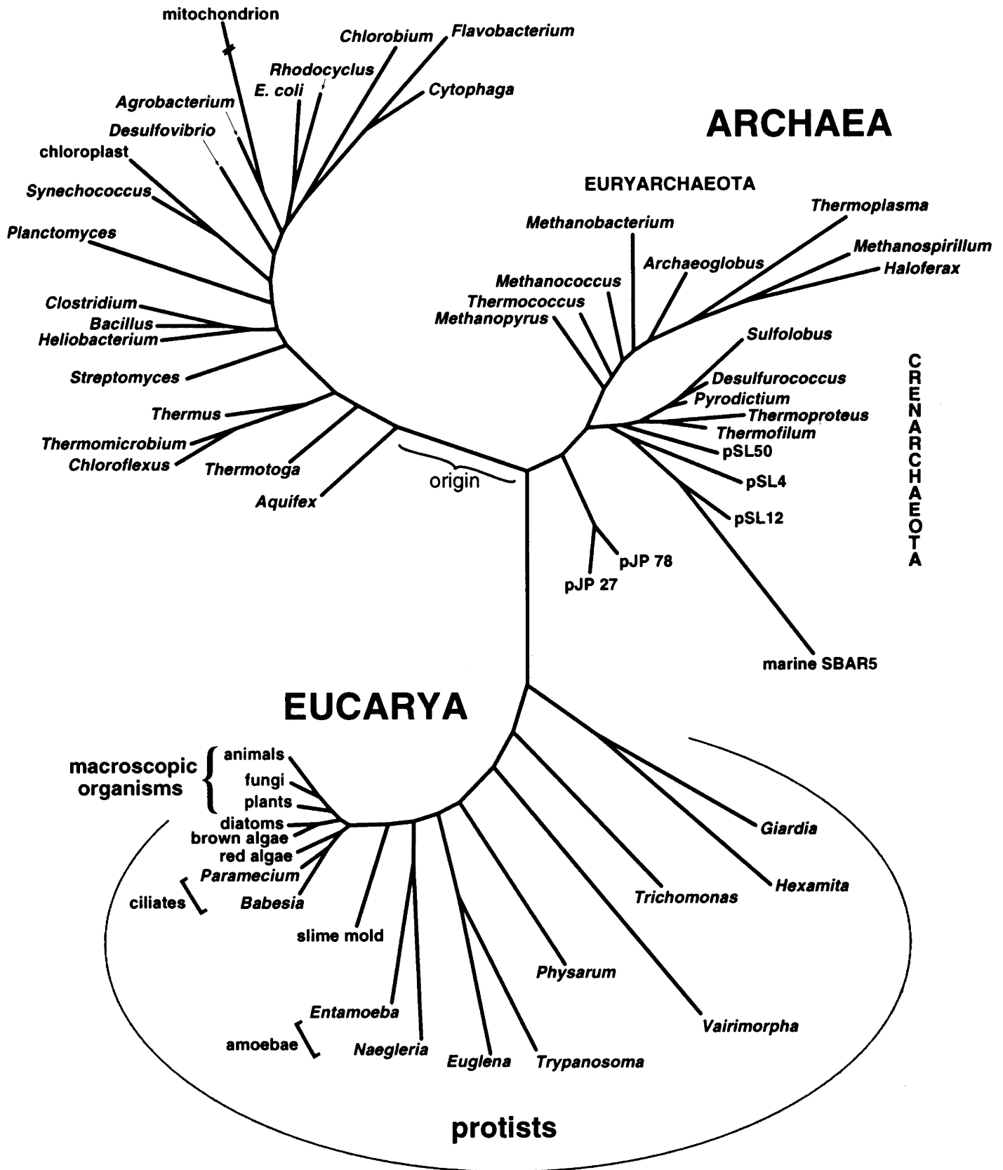
Figure 1. Diagrammatic “Universal” phylogenetic tree of life, based on small-subunit ribosomal RNA sequences. Based on analyses of Barns et al. (1996b), Olsen et al. (1994), and Sogin (1994).
