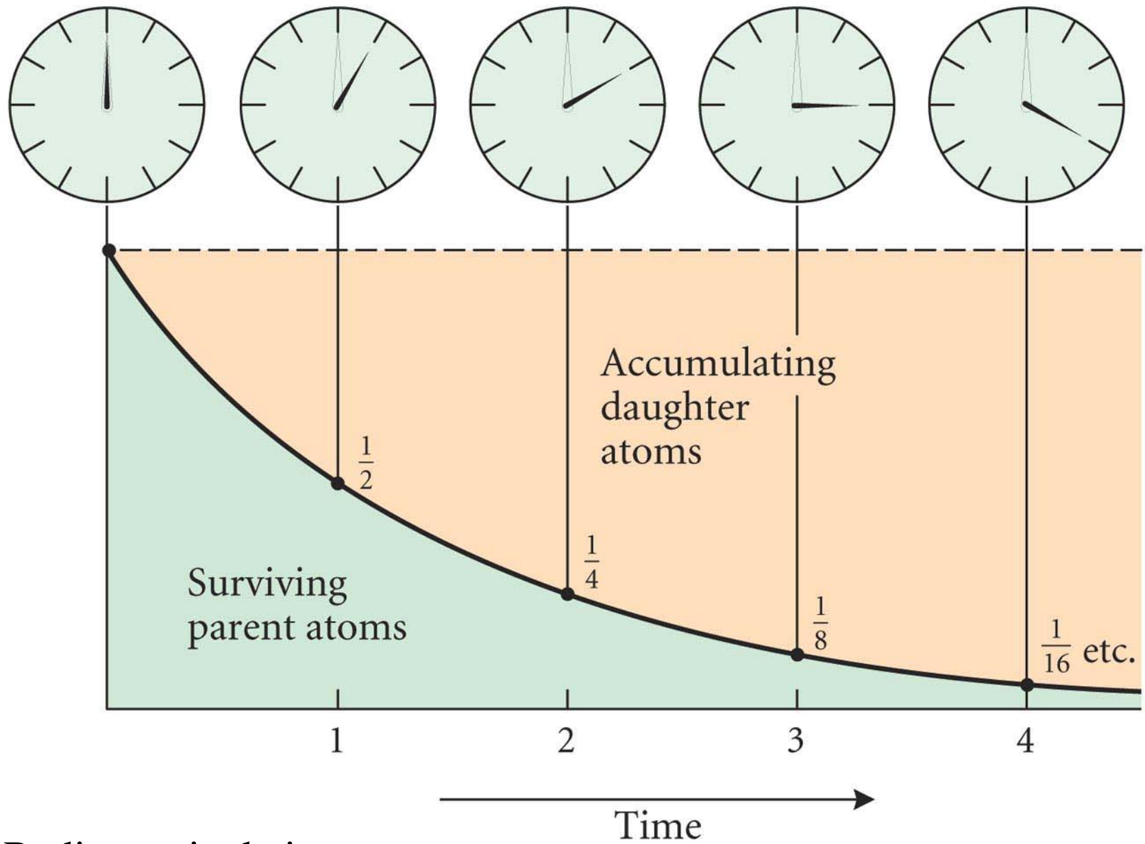
Radiometric dating
