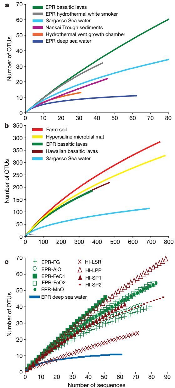
Figure 3 | Relative bacterial richness from several environmental studies shown through rarefaction analyses. a, Species richness of Bacteria inhabiting EPR seafloor lavas (cumulative results) is compared with that of other ocean environments, such as the Sargasso Sea 6 (partial curve), a MAR hydrothermal vent in situ growth chamber 7 , an EPR hydrothermal white smoker spire 5 , Nankai Trough deep-sea sediments 8 , and EPR deep sea water. The bacterial richness of the EPR basalts is also compared to a basalt-hosted community from Hawaii and other known high-richness environments (b), such as a farm soil 9 (partial curve) and a hypersaline microbial mat from the Guerrero Negro 10 (partial curve). Partial rarefaction curves are shown for visualization purposes, however complete data sets were used in calculating curve projections. c, Rarefaction curves for the individual EPR and Hawaii basalt clone libraries. Only partial curve is shown for HI-LPP (total clones = 246). Comparative studies in a and b are based on near full-length 16S rRNA gene sequences, and most studies are the sum of several environmental samples. OTUs are defined at a sequence similarity of \geq 97\% . FG = fresh glass; LSR = Loihi seamount South Rift; LPP = Loihi seamount Pisces Peak; SP1 & SP2 = South Point samples.
