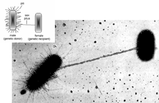
“Sex” Pili used in bacterial conjugation of E. coli cells
