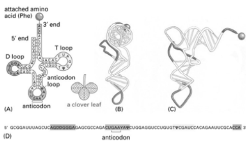
The structure of transfer RNA (tRNA)
