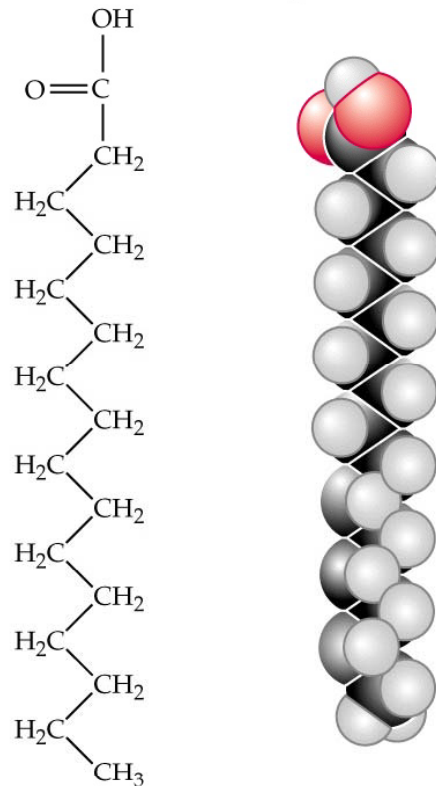
Palmitic acid
