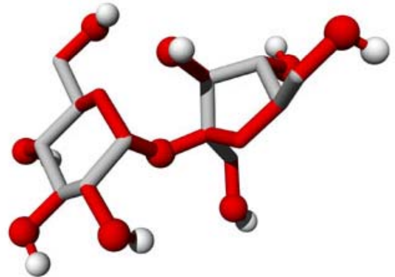
Sucrose
