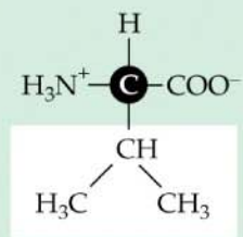
Valine
