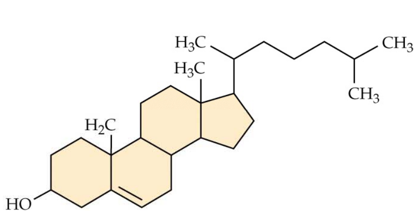
Cholesterol
