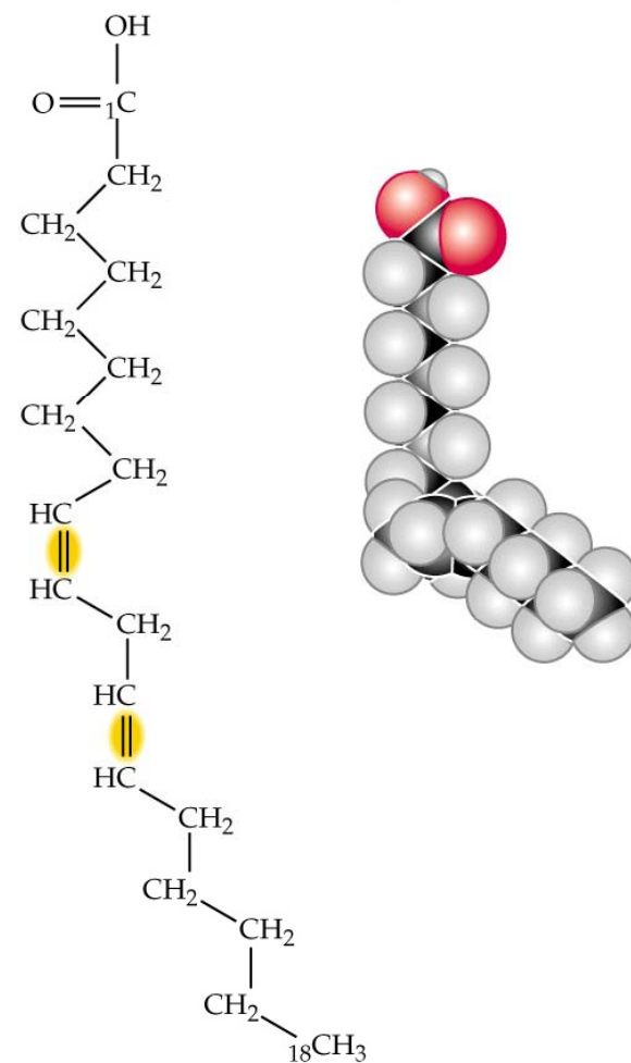
Linoleic acid
