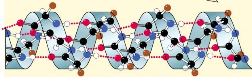
\alpha Helix
