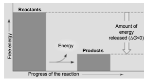
(a) Exergonic reaction: energy released
