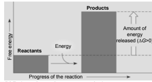
(b) Endergonic reaction: energy required
