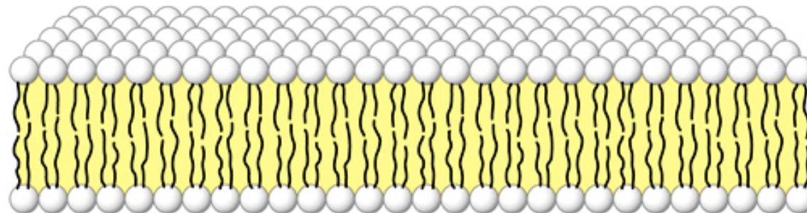
Phospholipid bilayer
